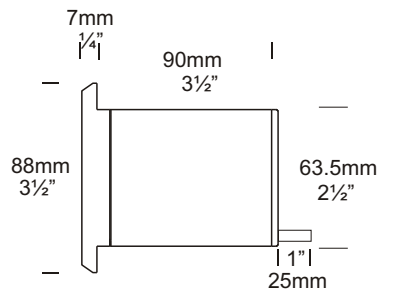
GU10 Option
